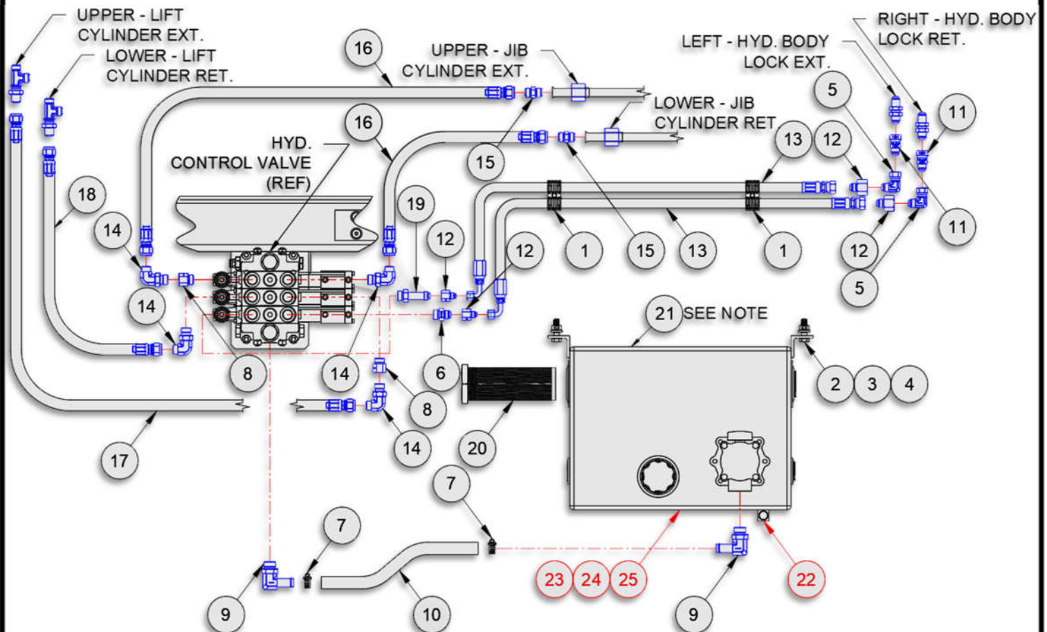
TANK CIRCUIT, 3-SECTION 418X/518X
