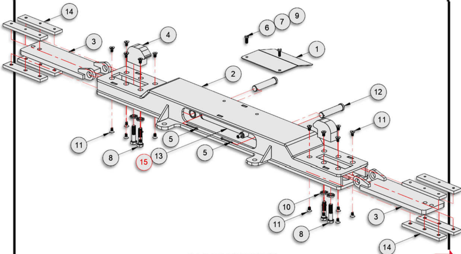
O-LOCK ASSEMBLY
