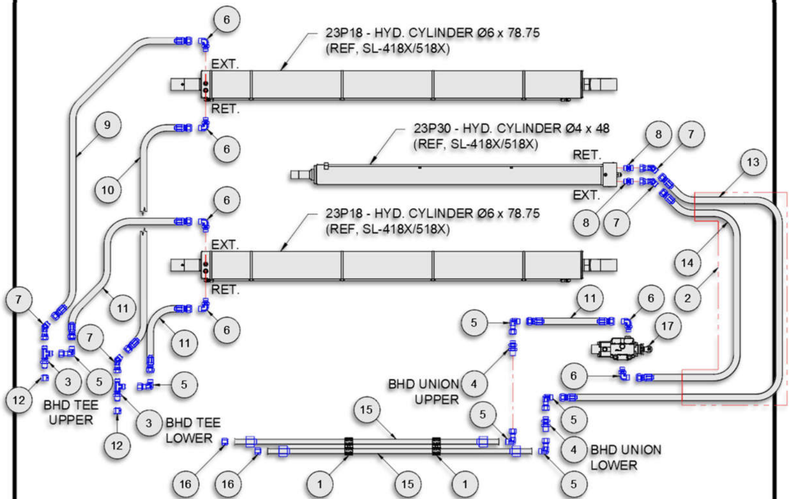
BASE CYLINDER CIRCUIT
