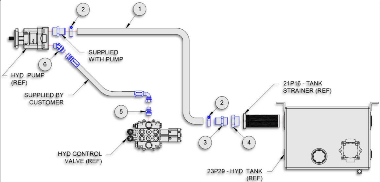
PUMP CIRCUIT
