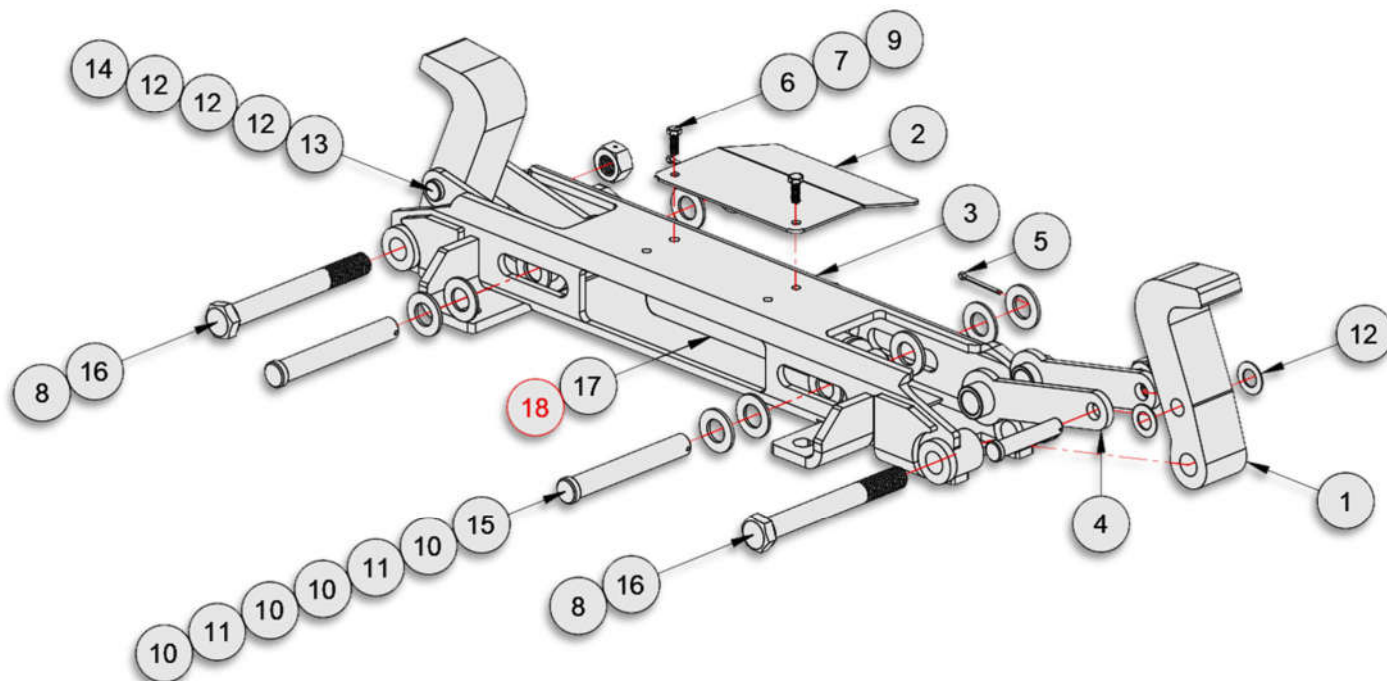
U-LOCK ASSEMBLY
