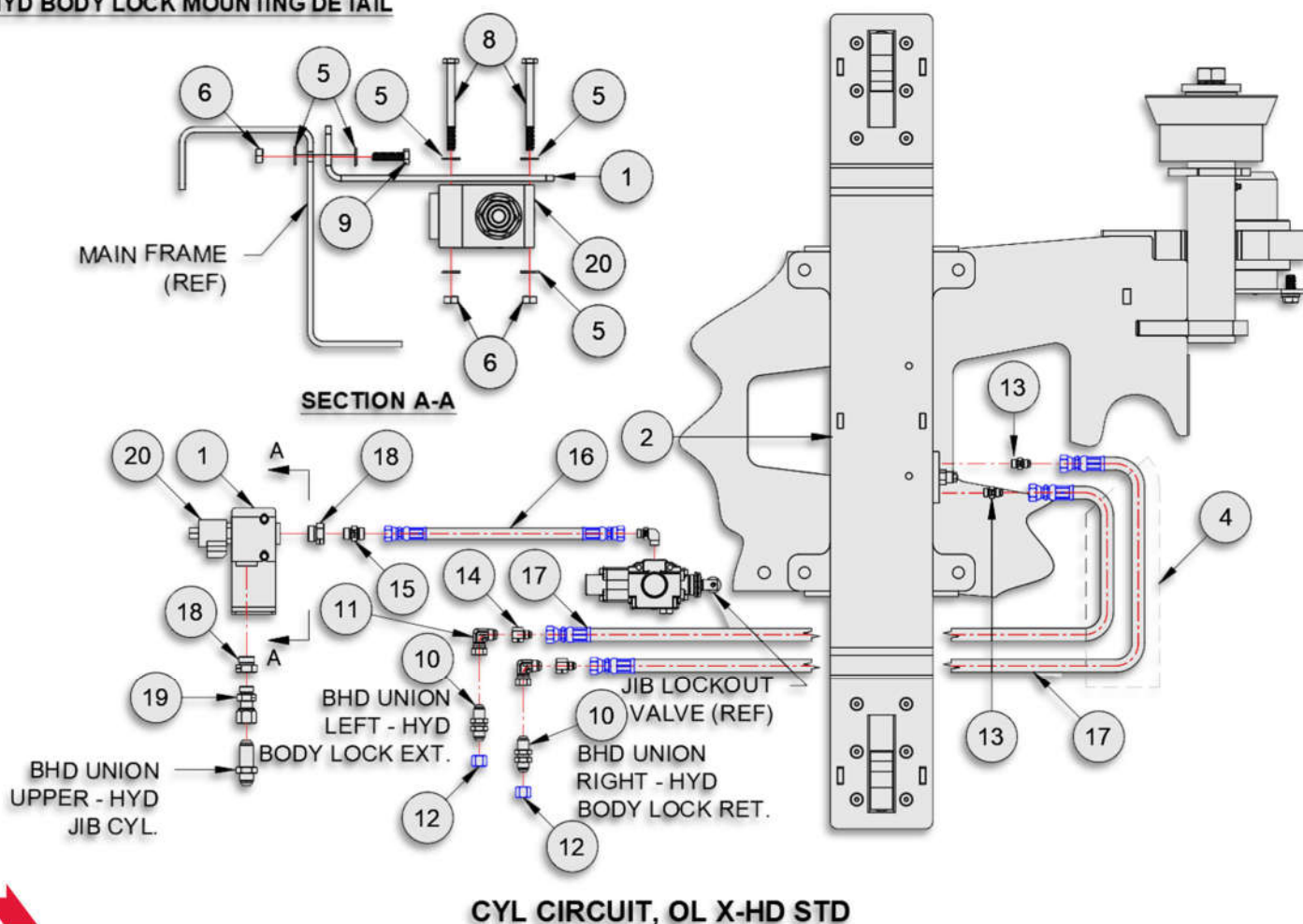
HYD BODY LOCK MOUNTING DETAIL
