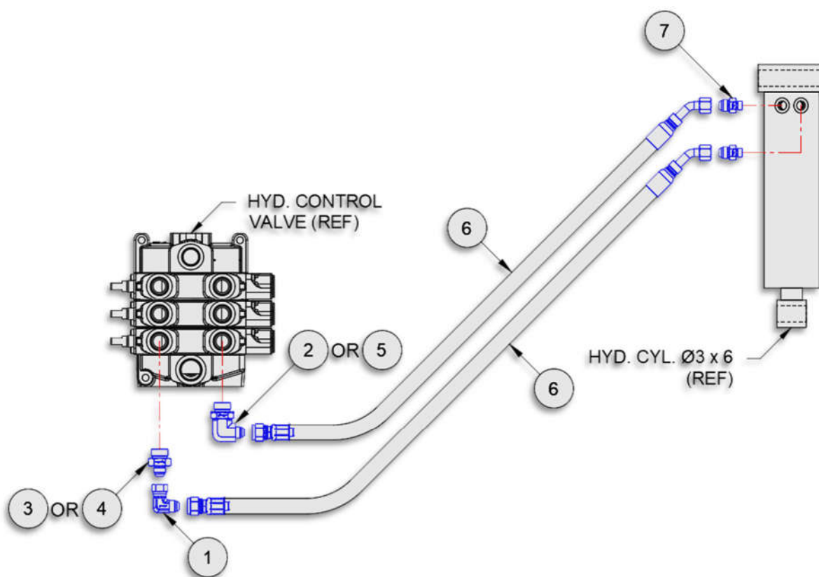
STABILIZER CIRCUIT
